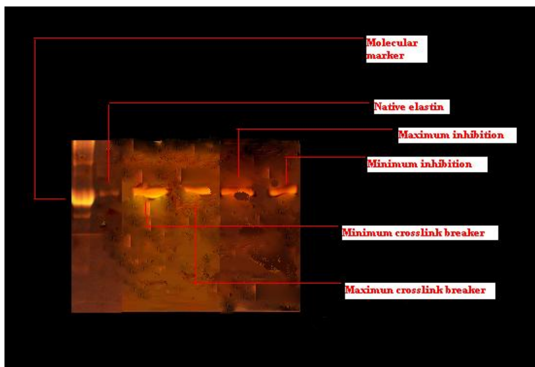
Fig-4 m-PAGE electrogram profiling to roots extracts in elastin protein reformation.
