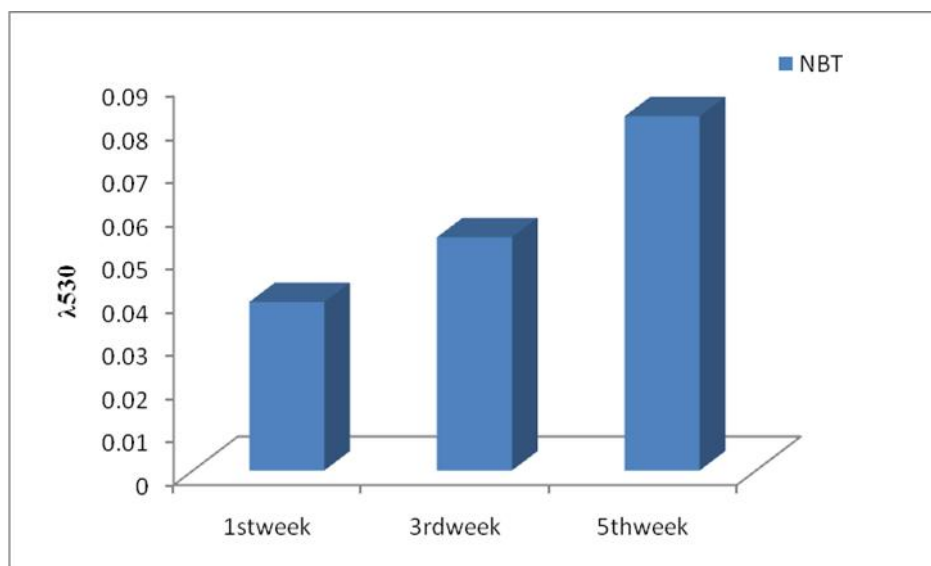
Fig: -2 Glycation level in different incubation period
