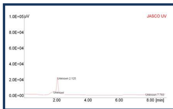
Fig-5: Calibration peak for Elastin (protein)
