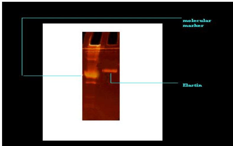
Fig:-1 .Electrogram of isolated elastin protein after polishing step with size exclusion chromatography.
