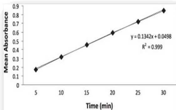
FIGURE 5 - Linearity curve of carvedilol in 6.8 citric-phosphate buffer with 1 % SLS.
