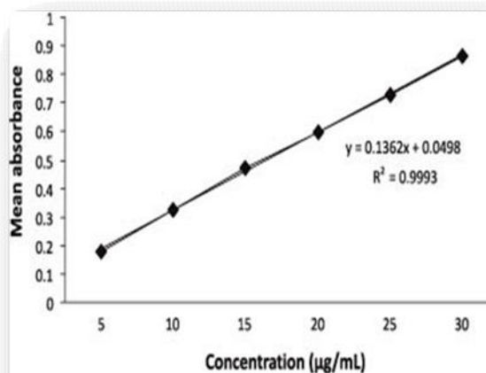
FIGURE 4 - Linearity curve of carvedilol in 0.1 N HCL.
